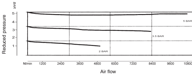
50 Series Pilot Operated Regulator (06,08)
